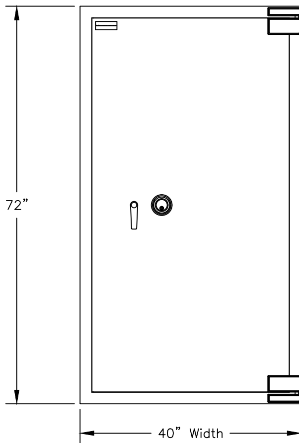
FRONT ELEVATION
